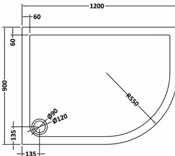
NTP115 - 1200 x 900 OFFSET QUADRANT TRAY RH
