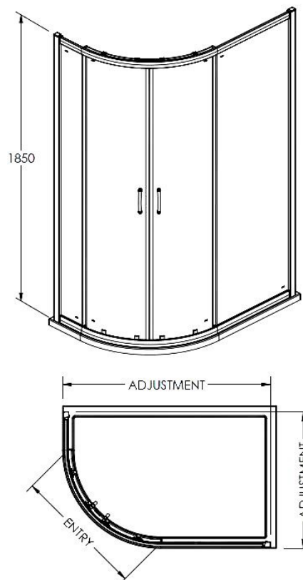
Ella Offset Quadrant Enclosure
