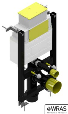
KEYTEC 0.82M WC FRAME WITH FRONT ACCESS DUAL FLUSH CISTERN H 780-980MM ADJ W 420MM ACC010 £314.00
