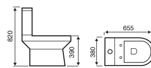
CLOSE COUPLED WC
