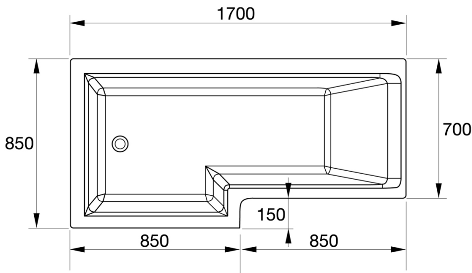
Drawings show left hand shower bath
