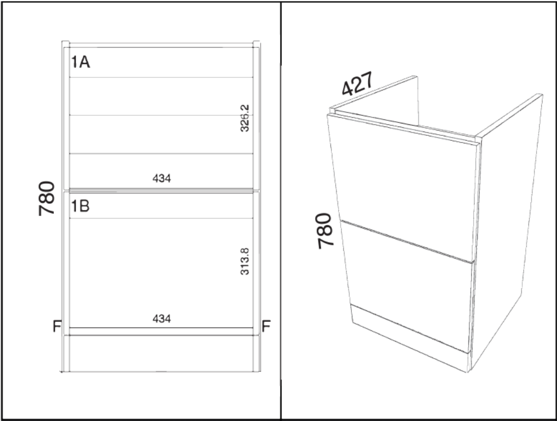
Technical drawing
