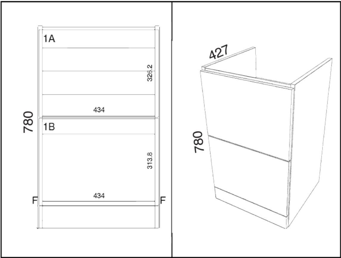
Technical drawing
