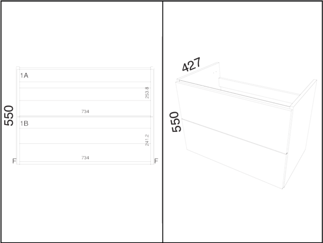
Technical drawing
