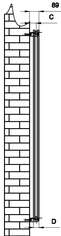
Side View
