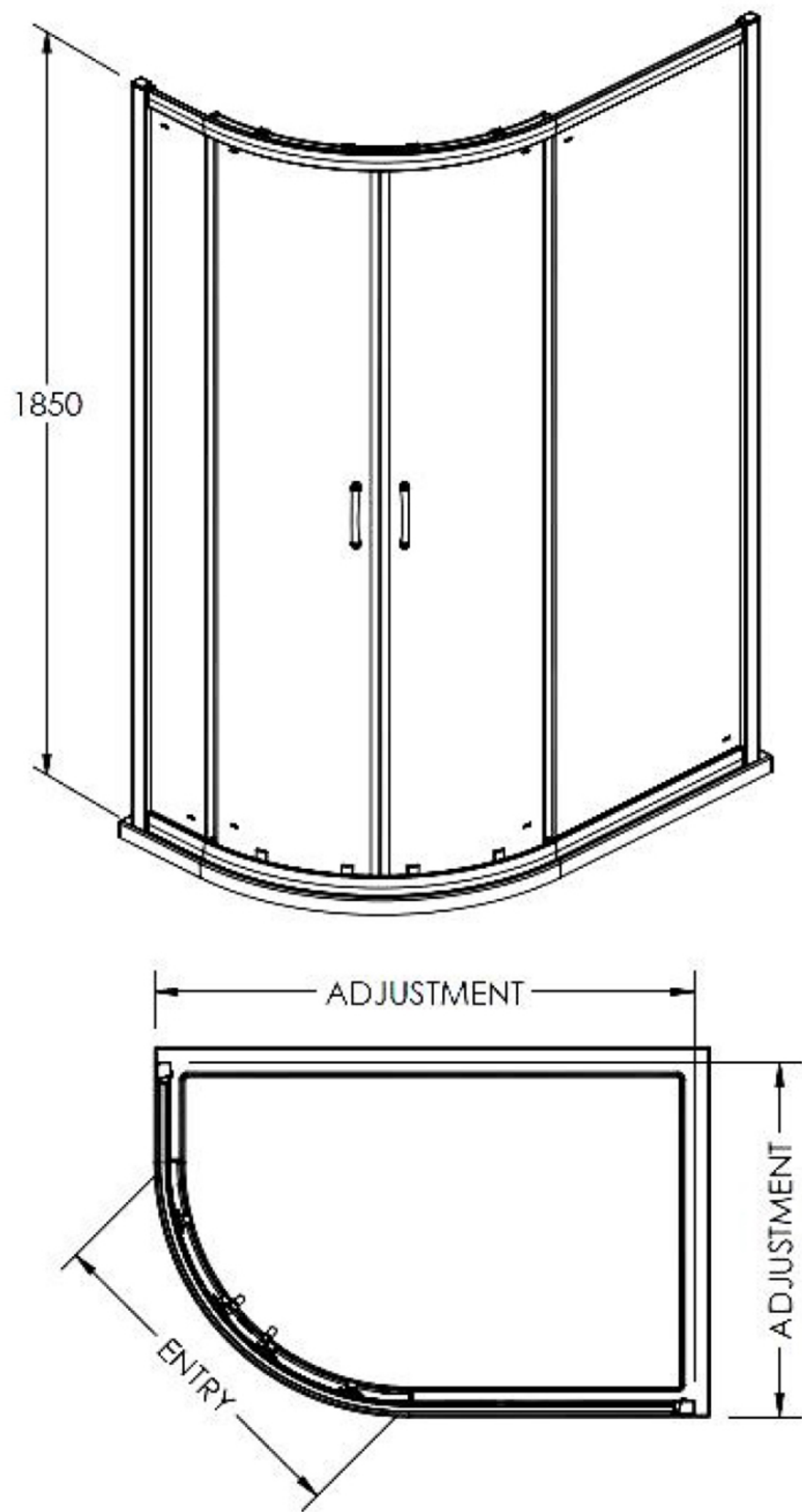
Ella Offset Quadrant Enclosure
