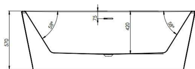
SECTION F-F SCALE 1 : 10
