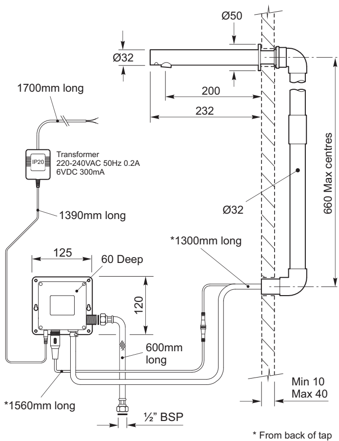
Sola wall mounted infra red spout, round
