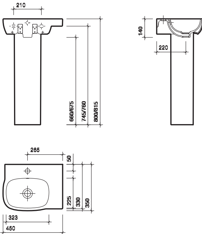
Moda handrinse 450 x 350mm, offset RH shelf
