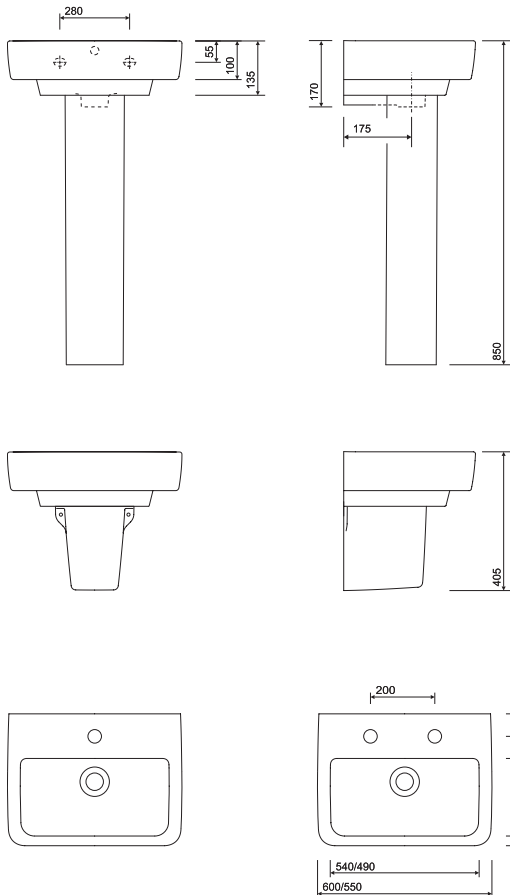
E200 550mm 1TH washbasin on pedestal
