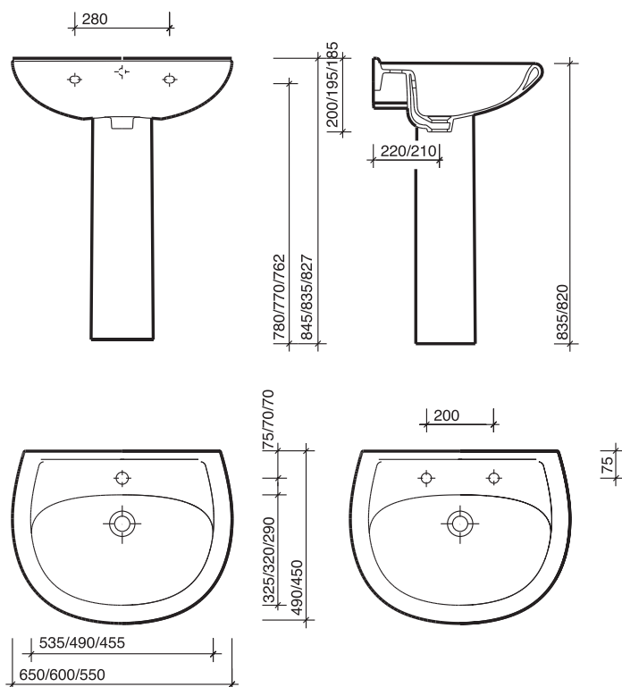
Galerie 650 x 510mm basin and pedestal
