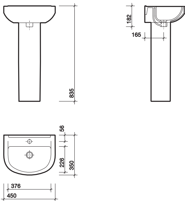
Refresh square 450 x 350mm handrinse basin and chrome bottle trap
