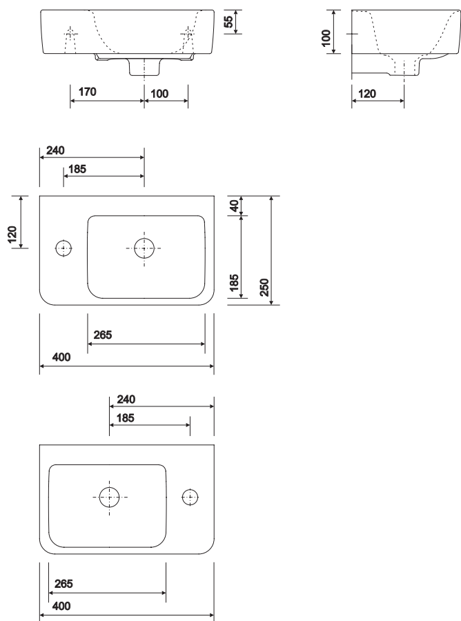
E200 400 x 250mm washbasin, with 1 RH Tap
