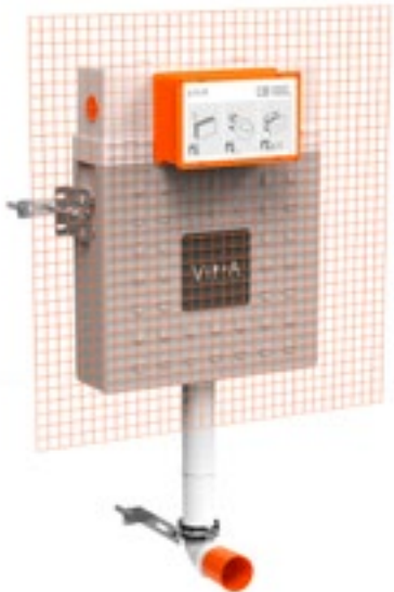
Concealed cistern 12cm, regular for back-to-wall WCs, 3/6 litre H: 730-830mm W: 420mm P: 120mm
