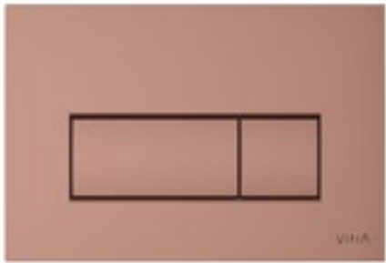
Loop Square mechanical flush plate compatible with all frames H: 165mm W: 244mm P: 9mm 740-2340 Soft Copper £85
