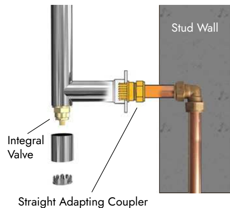
Integral Valve Fitting
