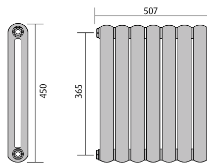
450mm High
